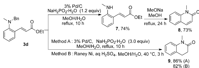
Scheme 4. Debenzylation of 3d .
